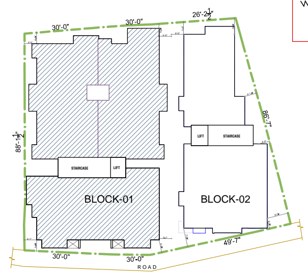
MASTER PLAN
