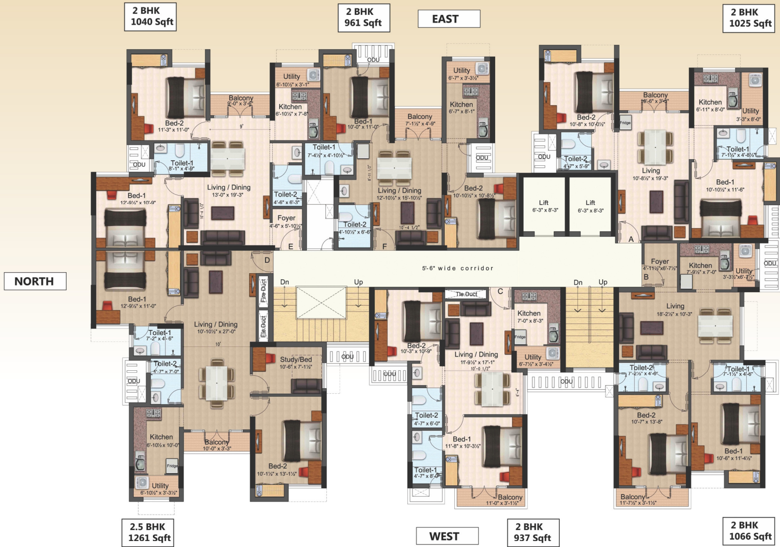
Tower - 3 Second - Sixteenth Typical Floor Plan
